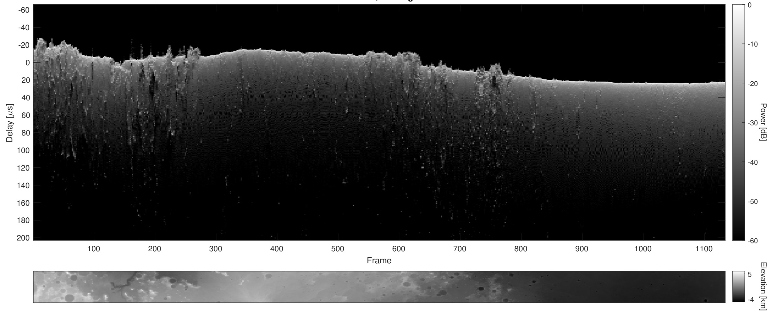
Orbit 20812, Cluttergram
