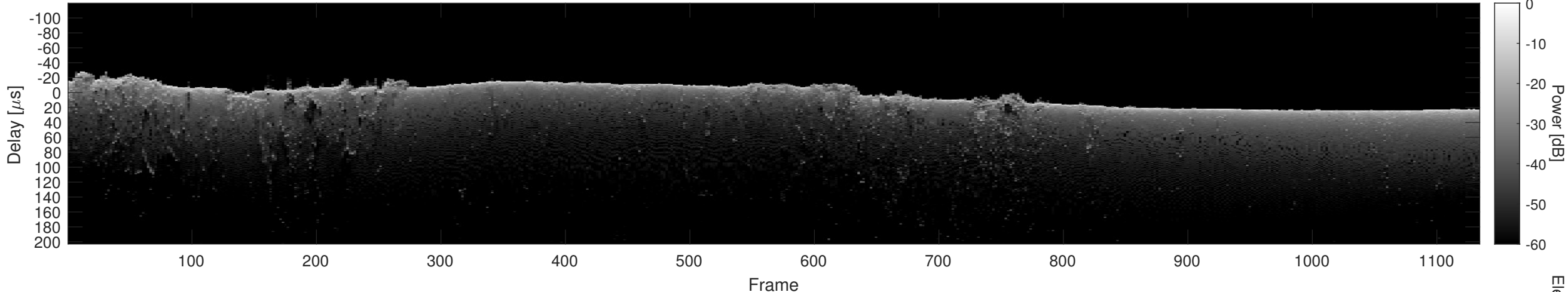
Orbit 20812, Cluttergram
