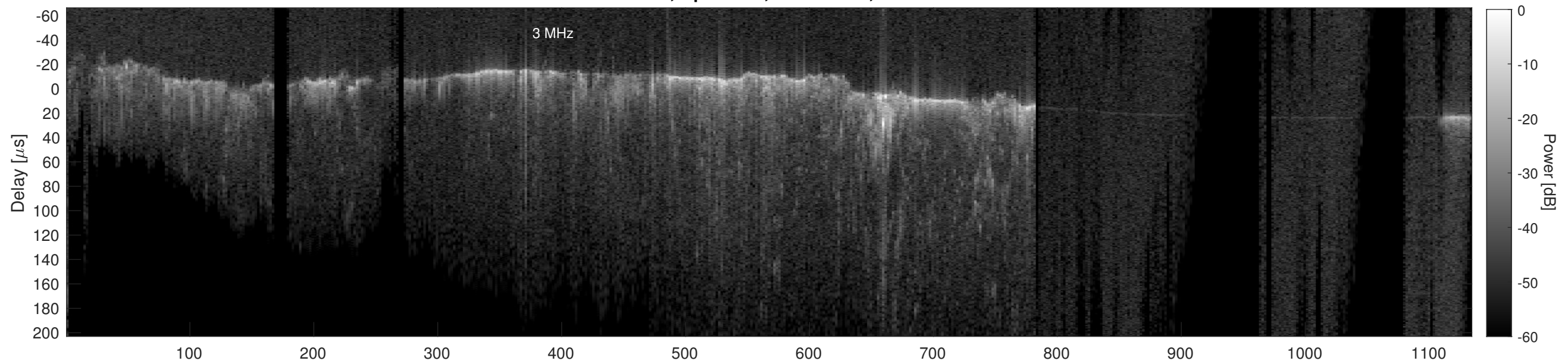
Orbit 20812, Cluttergram
