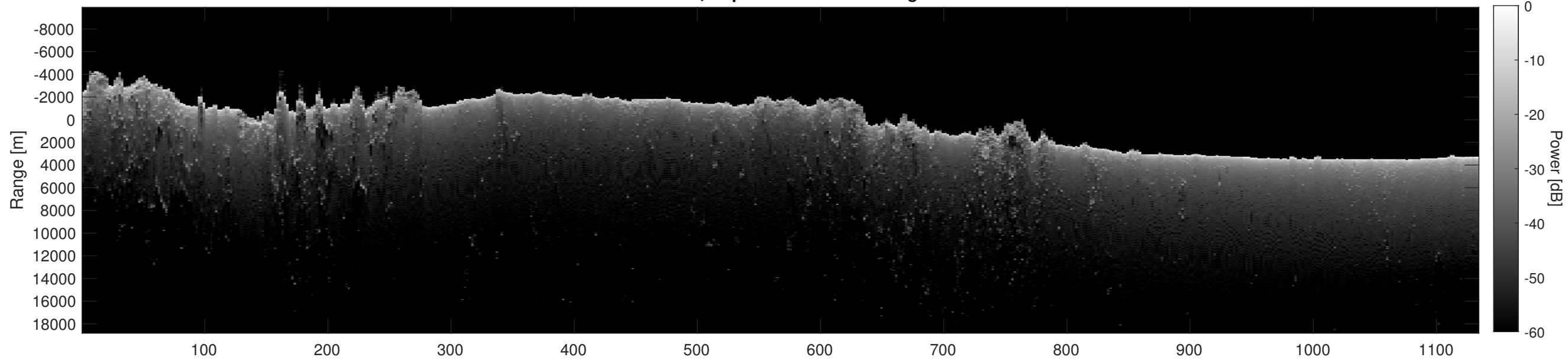
Orbit 20812, Depth-Corrected Cluttergram
