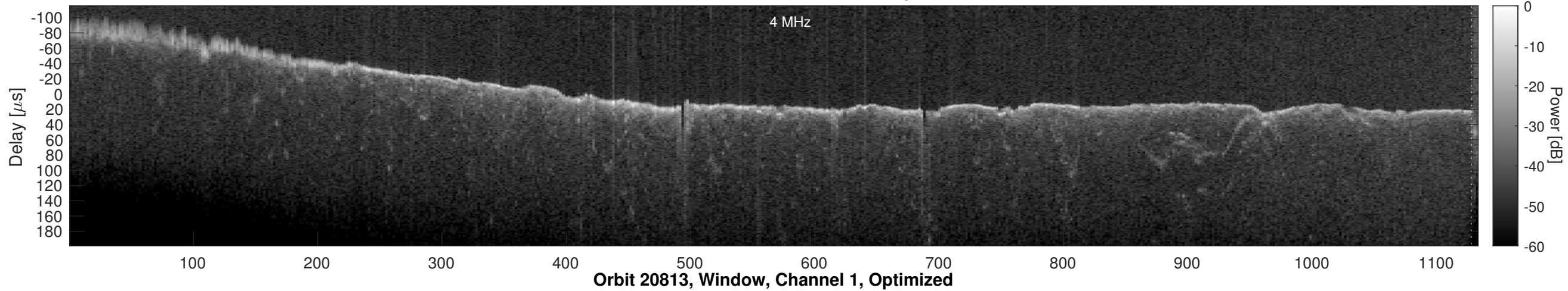
Orbit 20813, Window, Channel 1, Chapman
