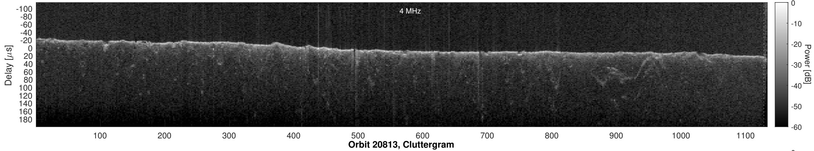
Orbit 20813, Window, Channel 1, Optimized
