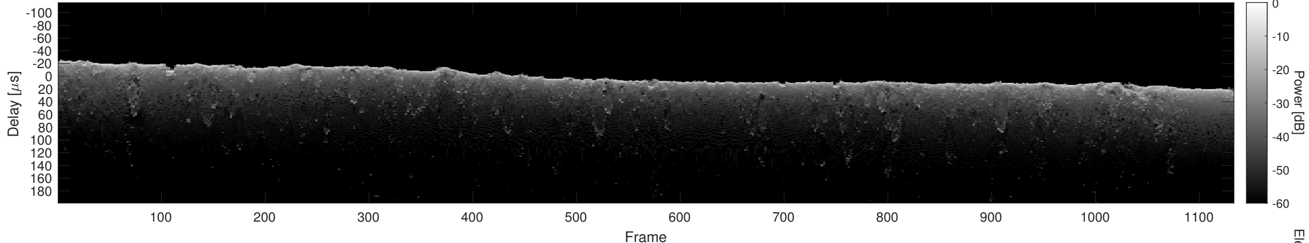
Orbit 20813, Cluttergram
