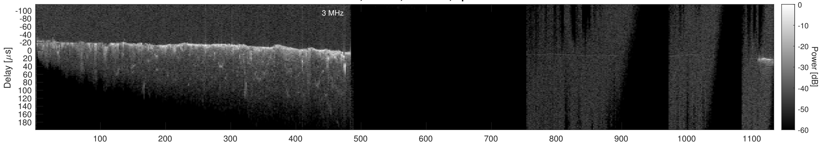
Orbit 20813, Cluttergram
