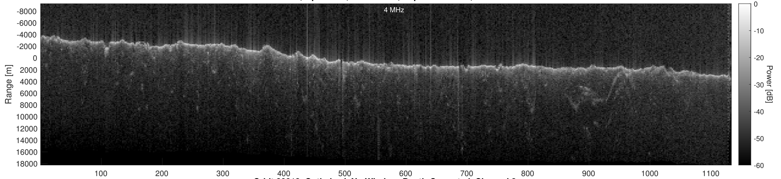
Orbit 20813, Optimized, No Window, Depth-Corrected, Channel 2
