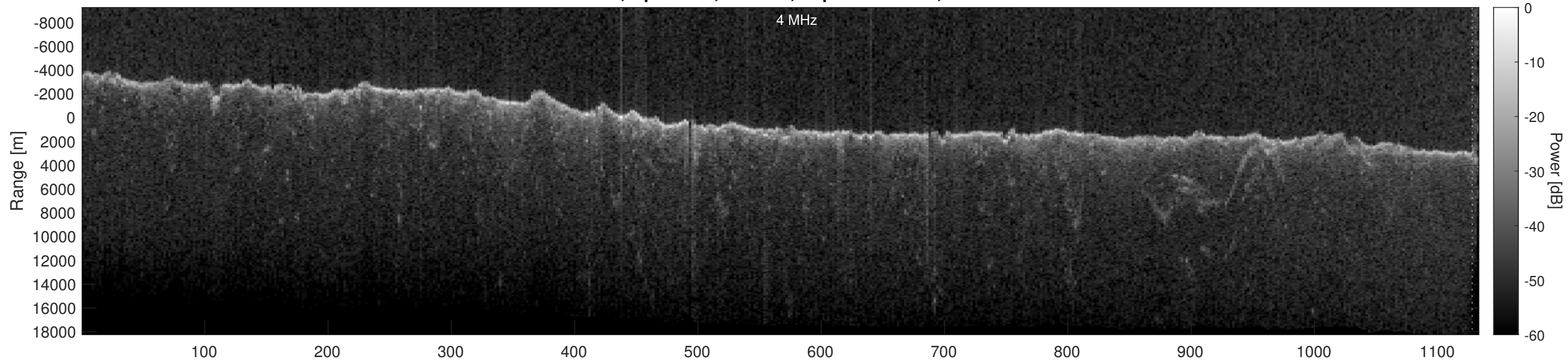
Orbit 20813, Optimized, Window, Depth-Corrected, Channel 2
