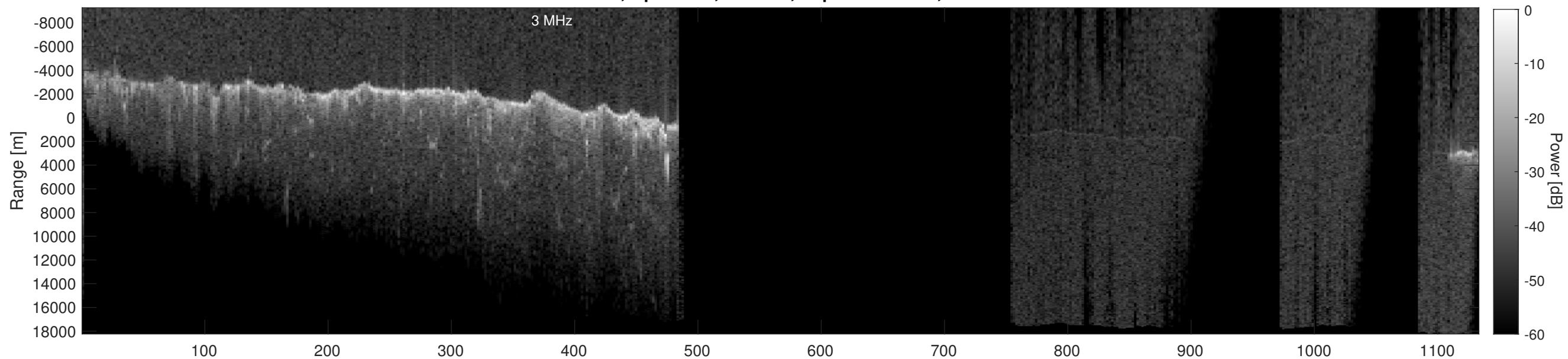
Orbit 20813, Depth-Corrected Cluttergram
