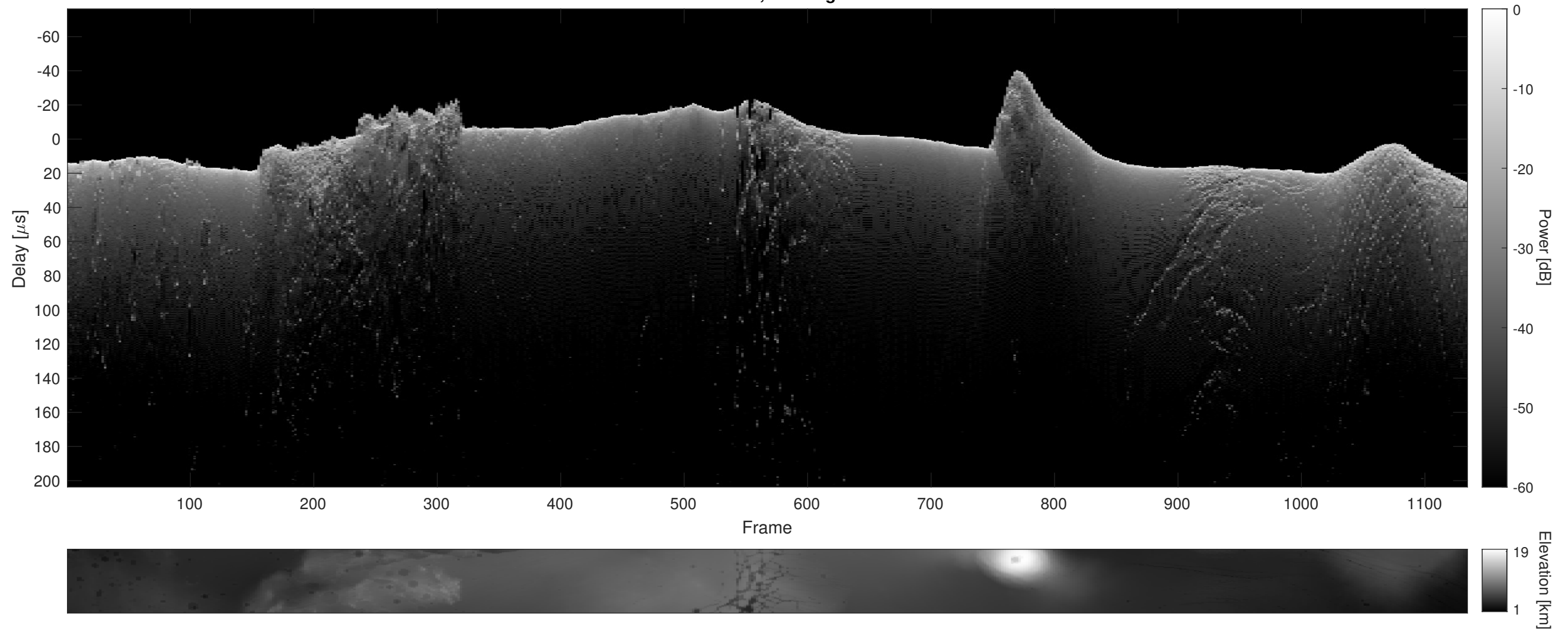
Orbit 20814, Cluttergram
