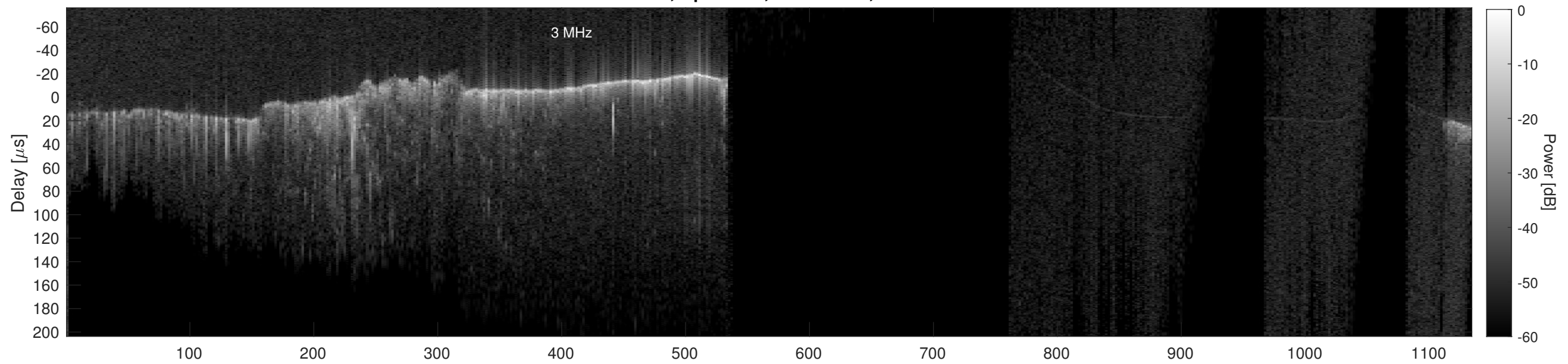
Orbit 20814, Cluttergram
