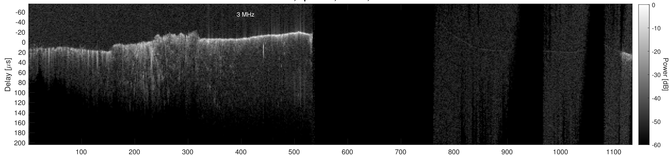
Orbit 20814, Cluttergram
