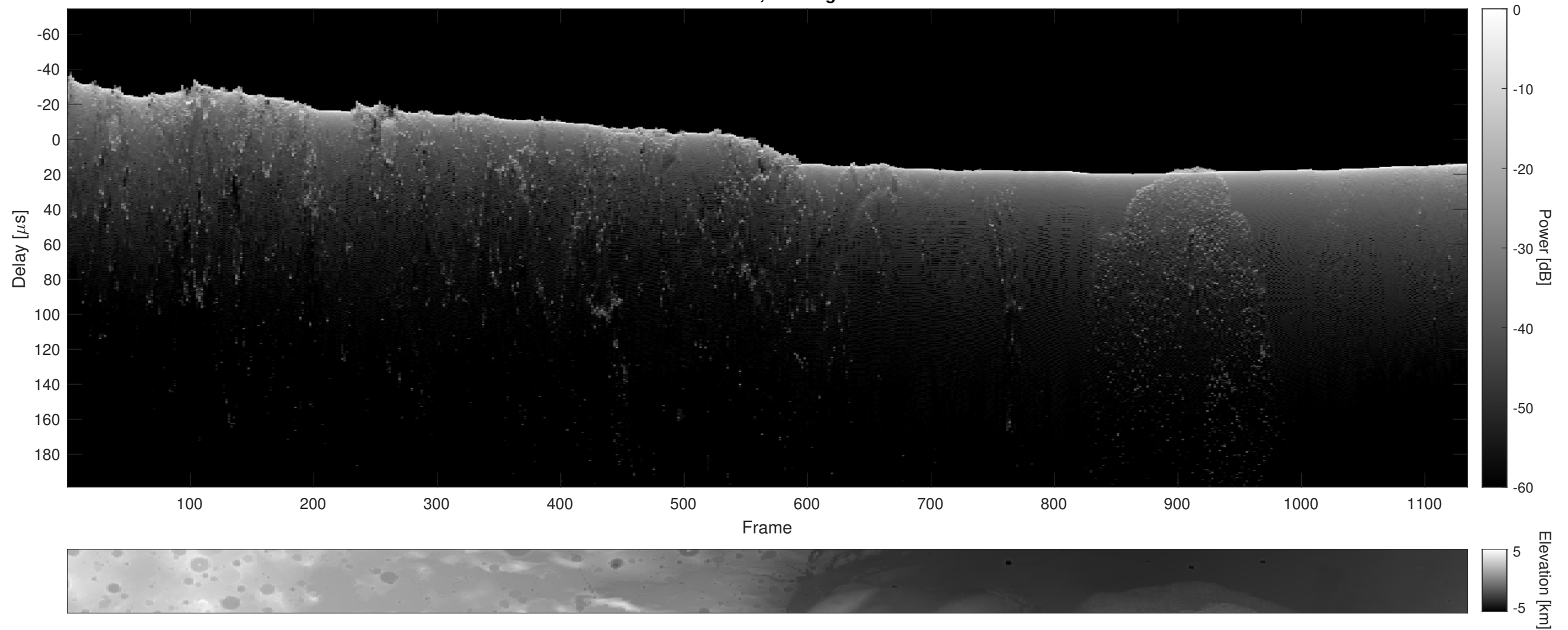
Orbit 20818, Cluttergram
