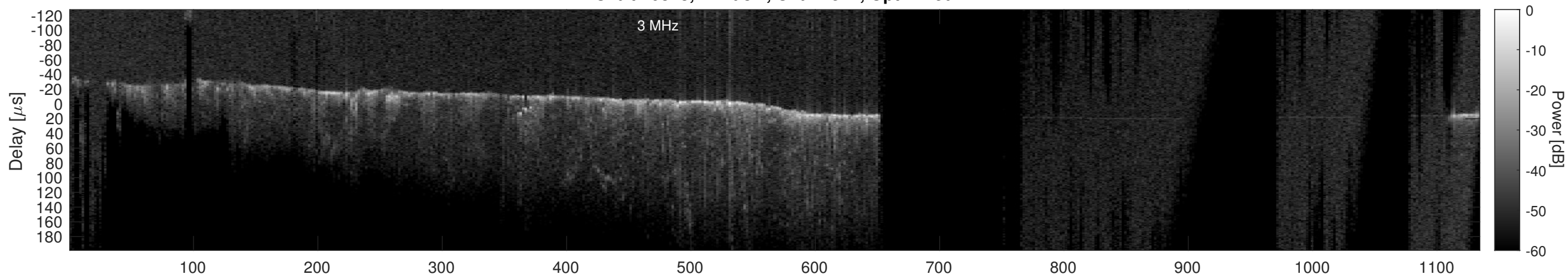
Orbit 20818, Cluttergram
