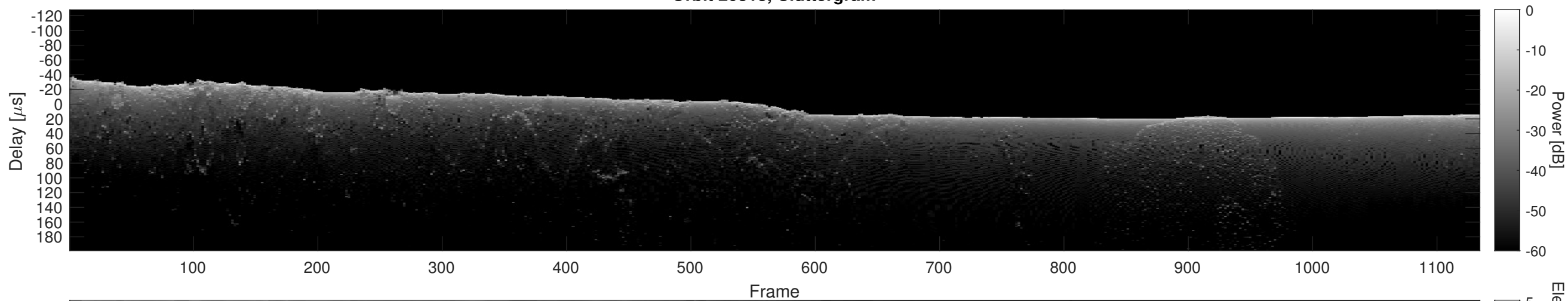
Orbit 20818, Cluttergram
