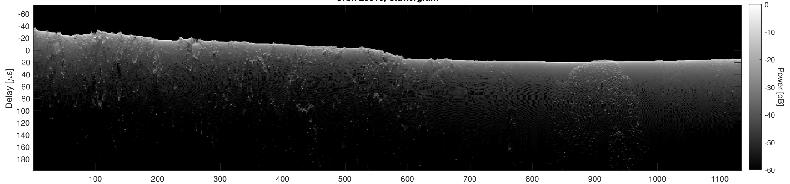
Orbit 20818, Cluttergram
