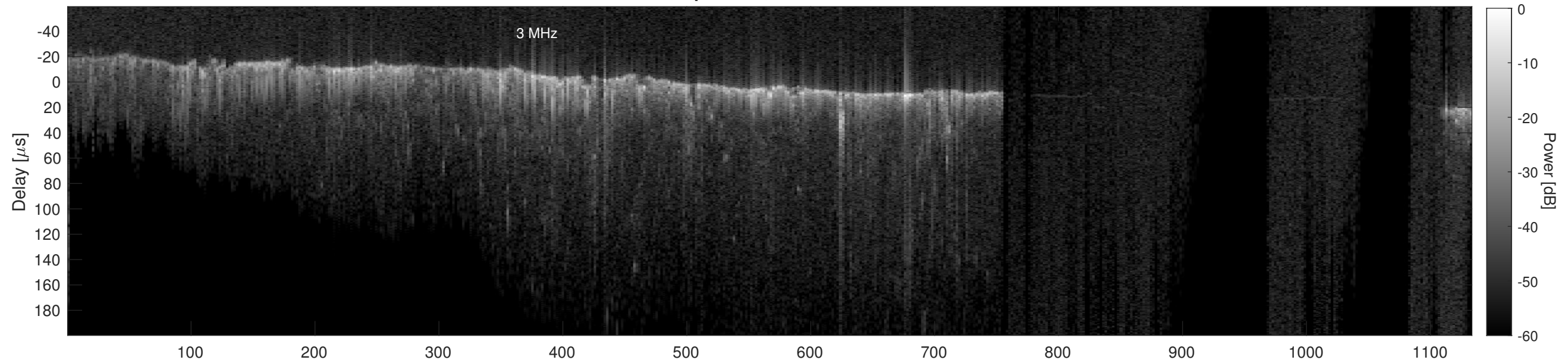
Orbit 20820, Cluttergram
