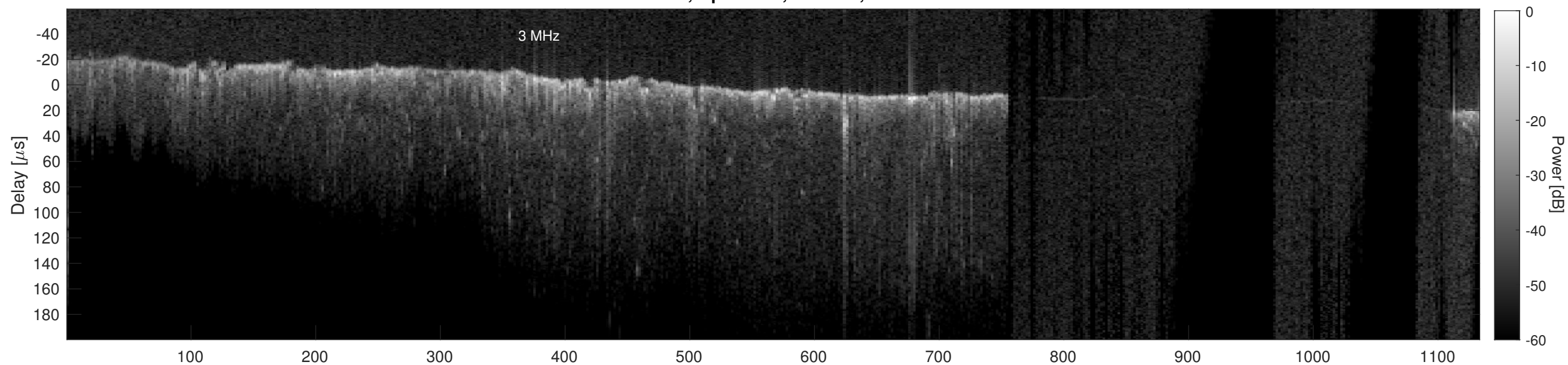
Orbit 20820, Cluttergram
