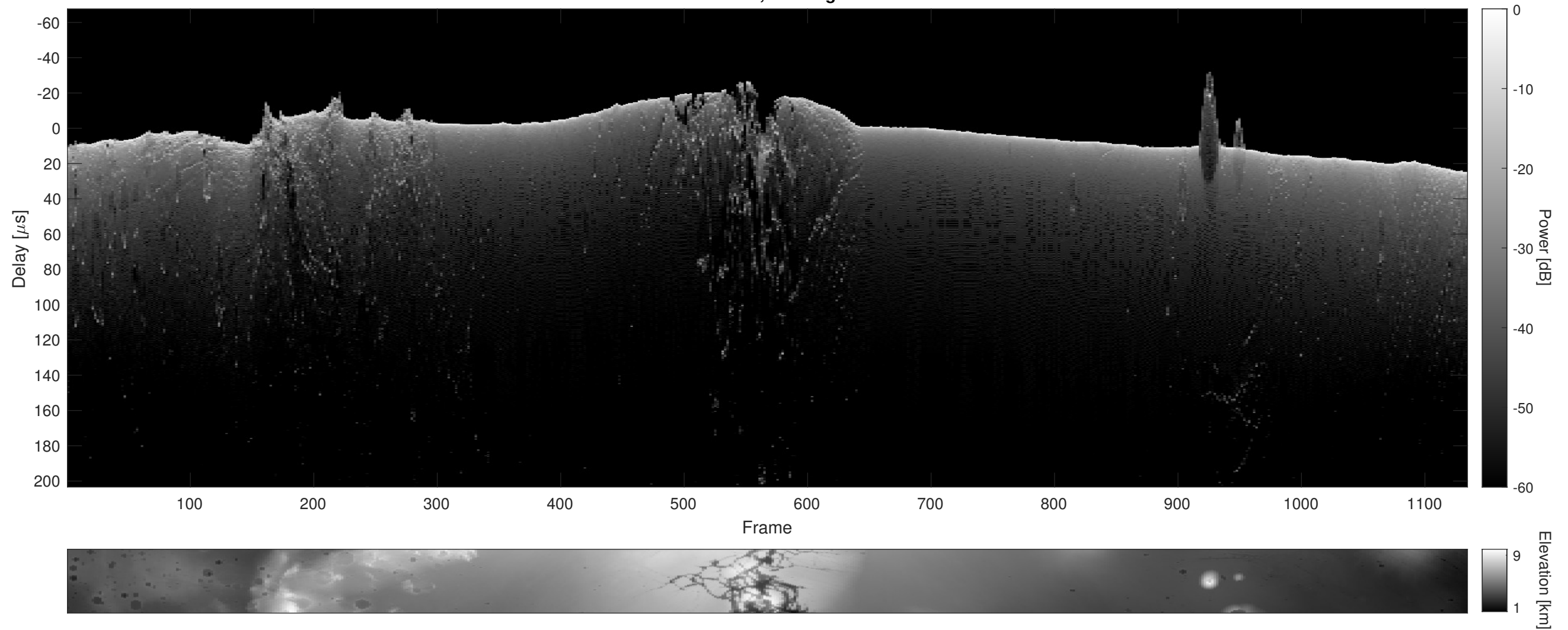
Orbit 20821, Cluttergram
