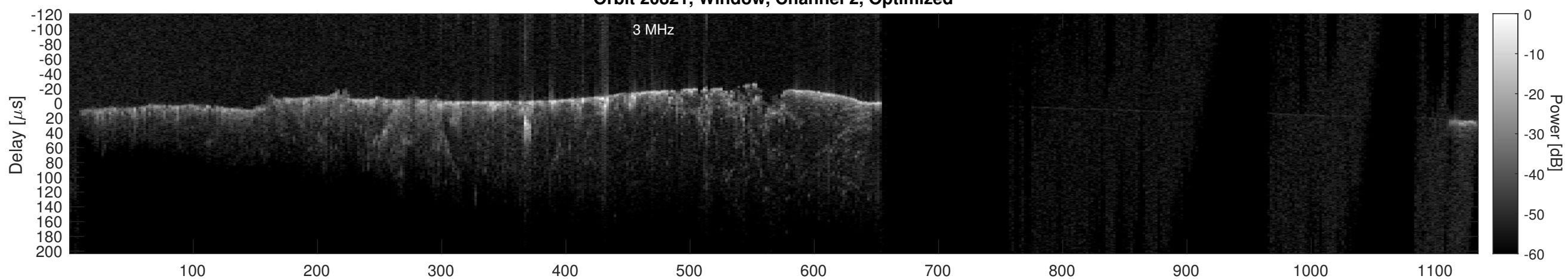
Orbit 20821, Cluttergram
