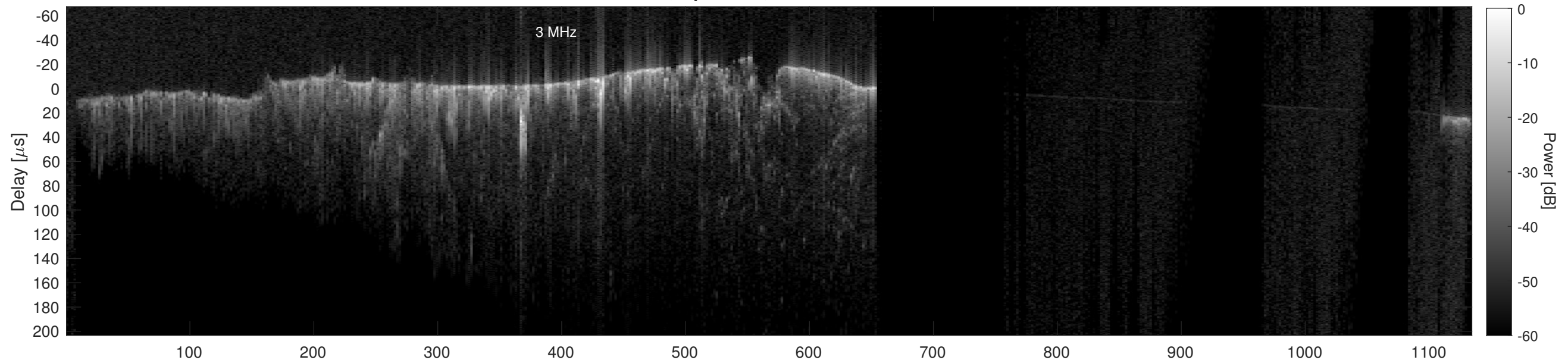
Orbit 20821, Cluttergram
