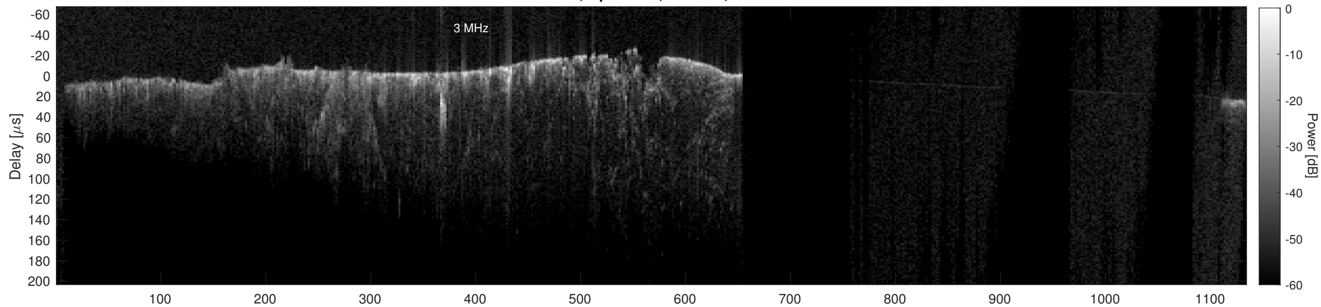
Orbit 20821, Cluttergram
