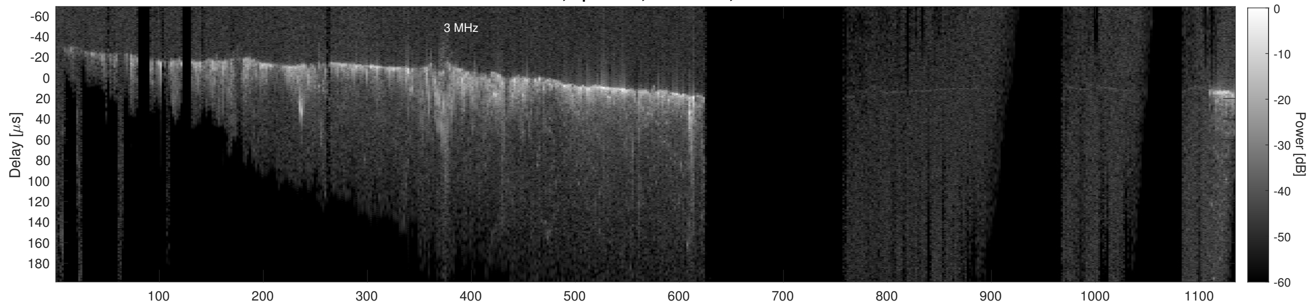
Orbit 20822, Cluttergram
