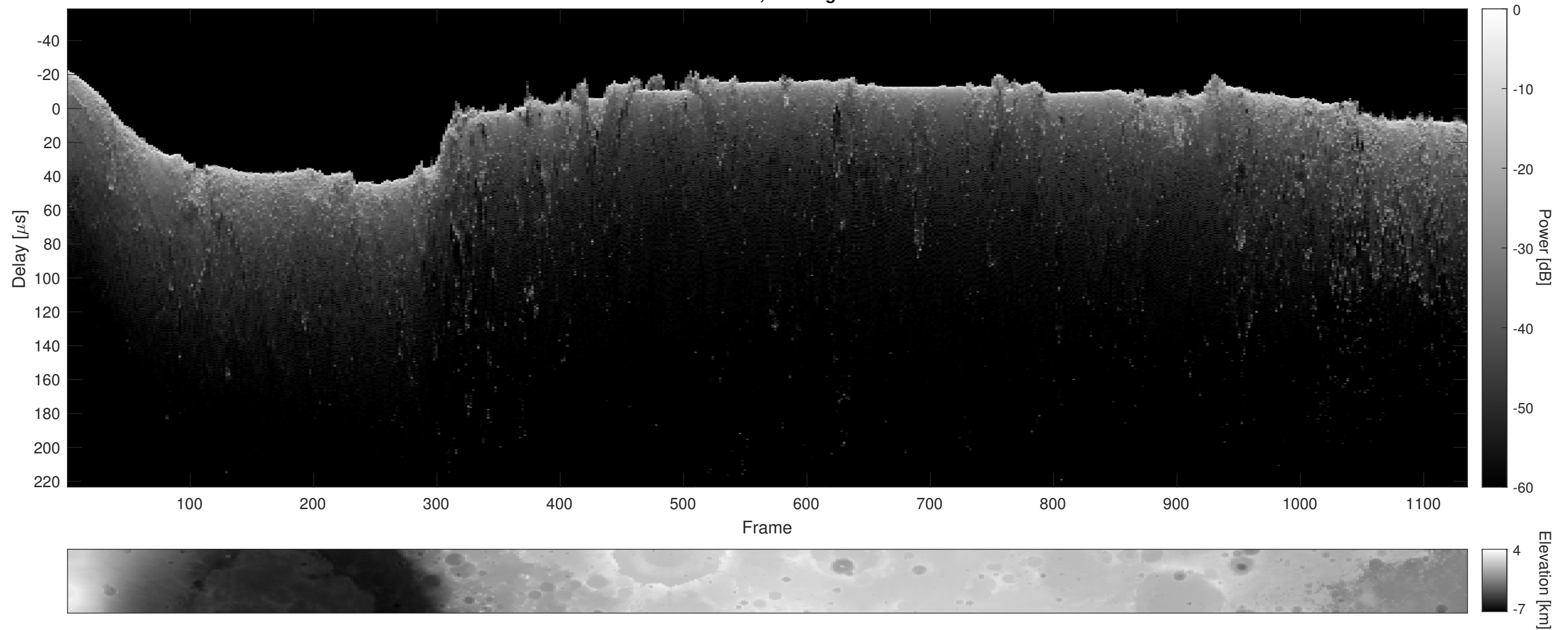
Orbit 20823, Cluttergram
