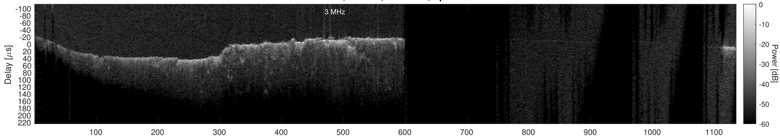
Orbit 20823, Cluttergram
