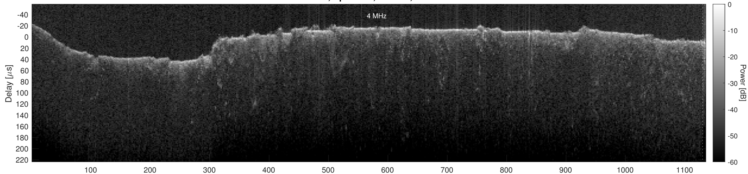
Orbit 20823, Optimized, Window, Channel 2
