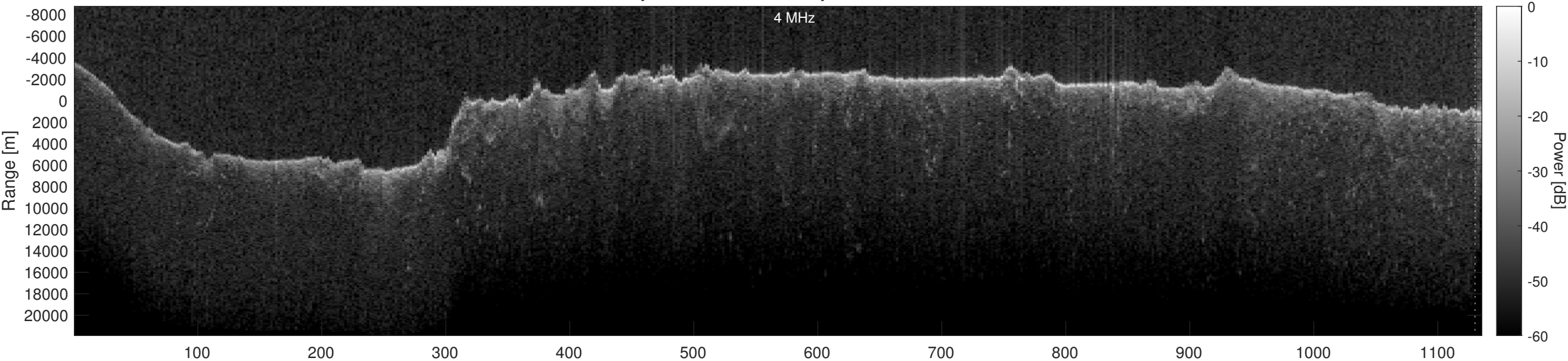
Orbit 20823, Optimized, Window, Depth-Corrected, Channel 2
