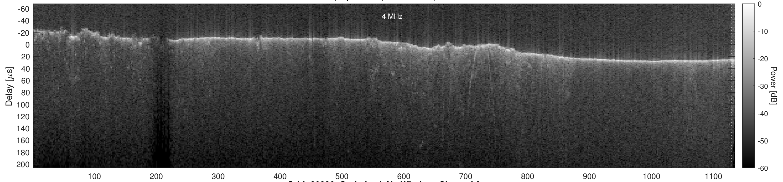
Orbit 20826, Optimized, No Window, Channel 2
