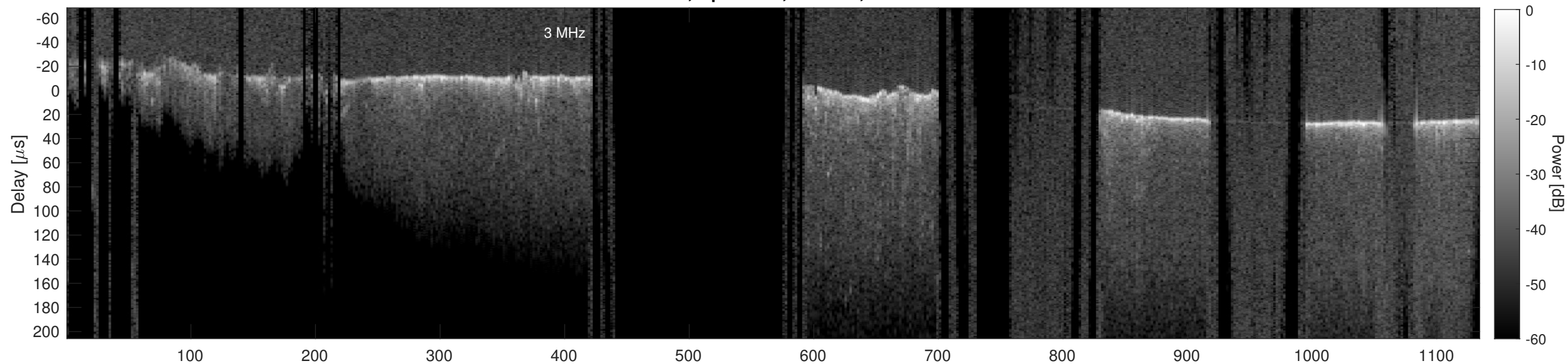
Orbit 20826, Cluttergram
