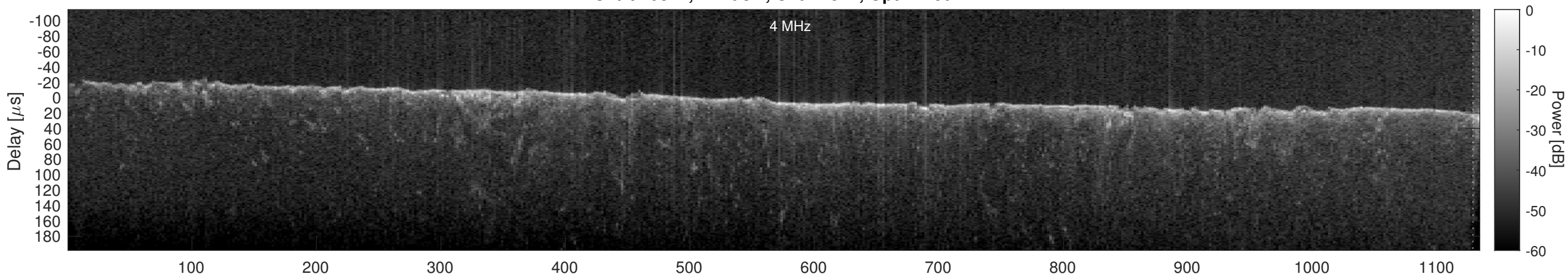
Orbit 20827, Cluttergram
