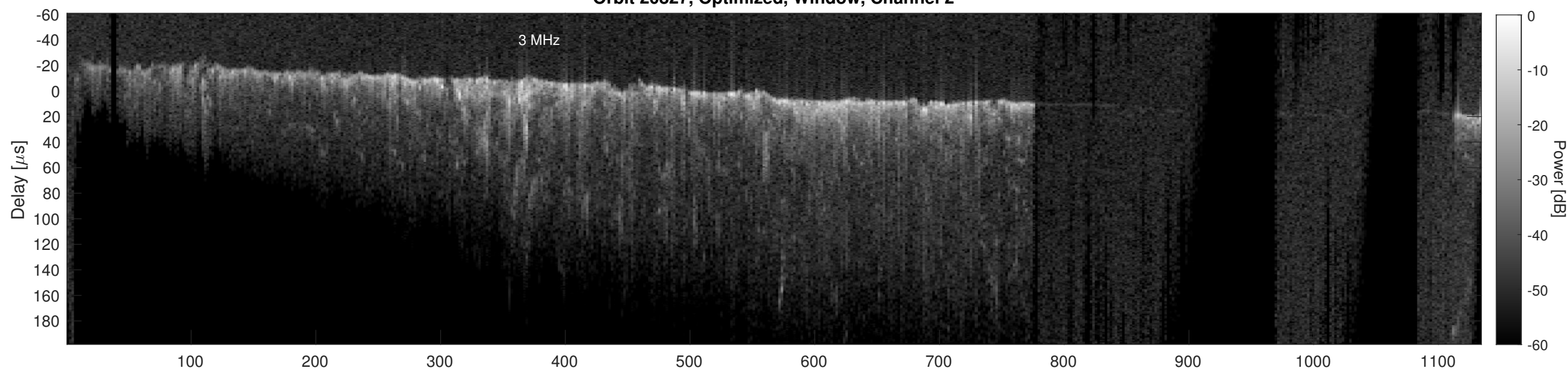
Orbit 20827, Cluttergram
