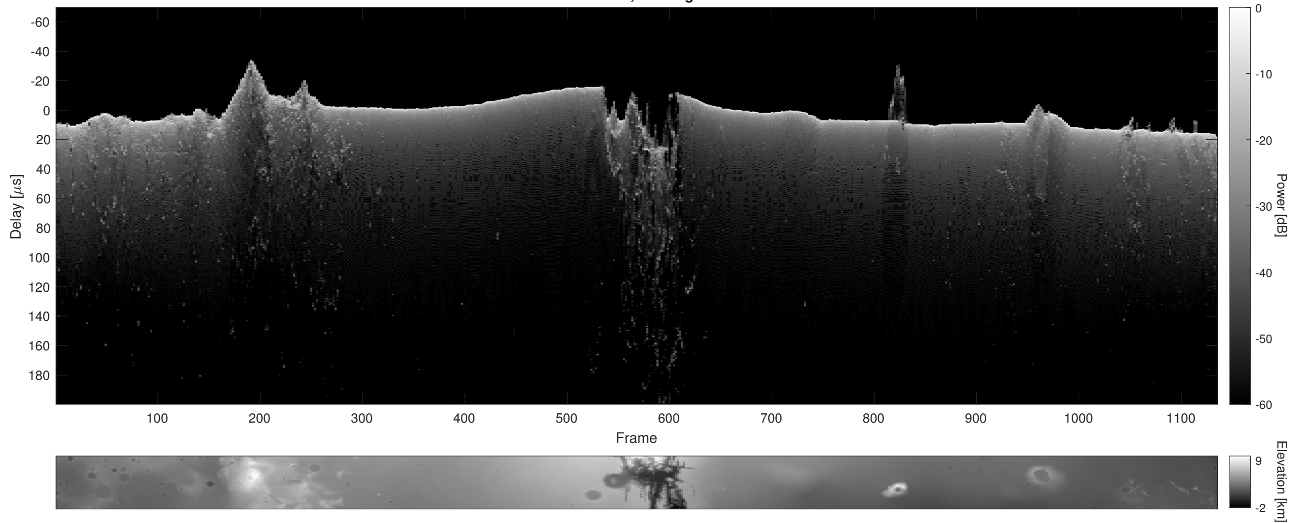
Orbit 20828, Cluttergram
