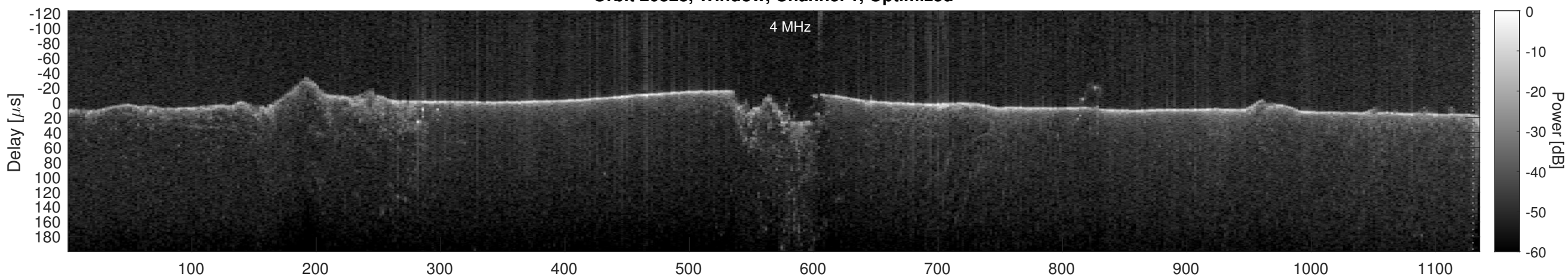
Orbit 20828, Cluttergram
