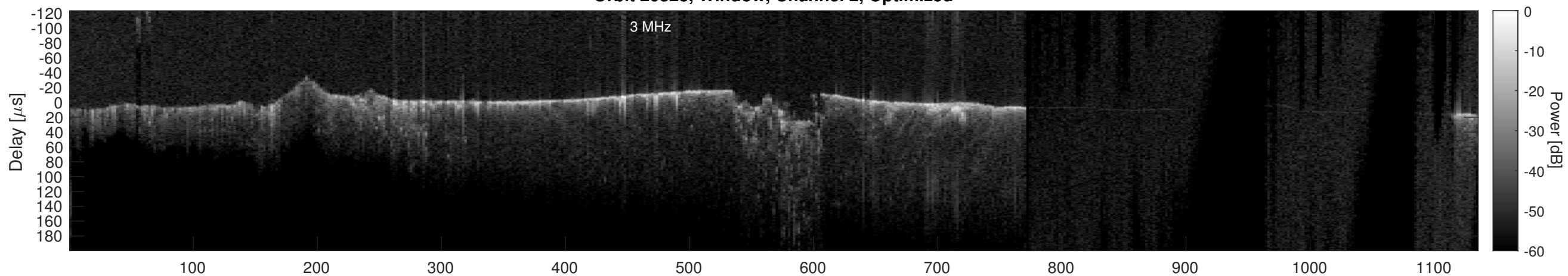
Orbit 20828, Cluttergram
