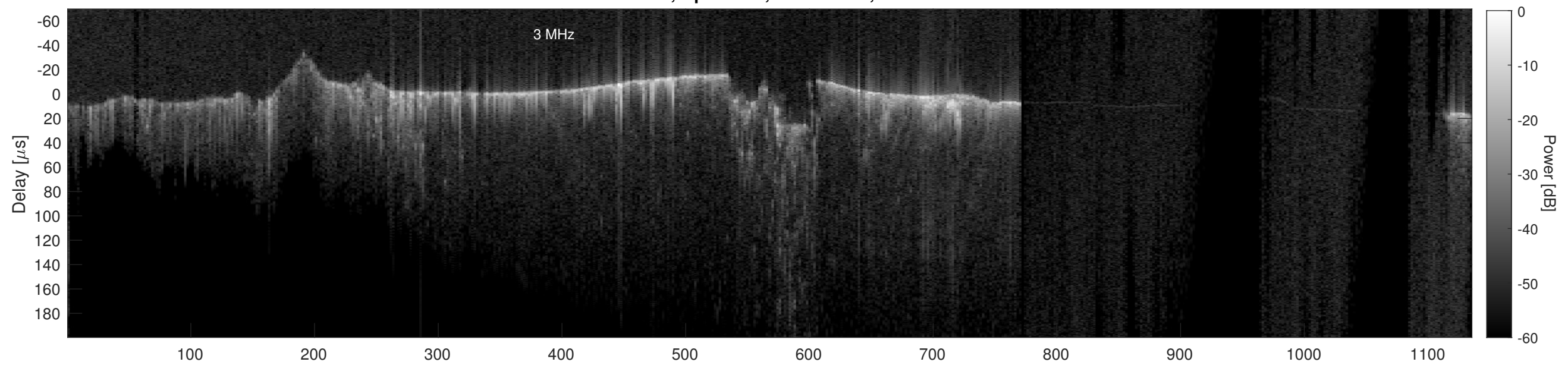
Orbit 20828, Cluttergram
