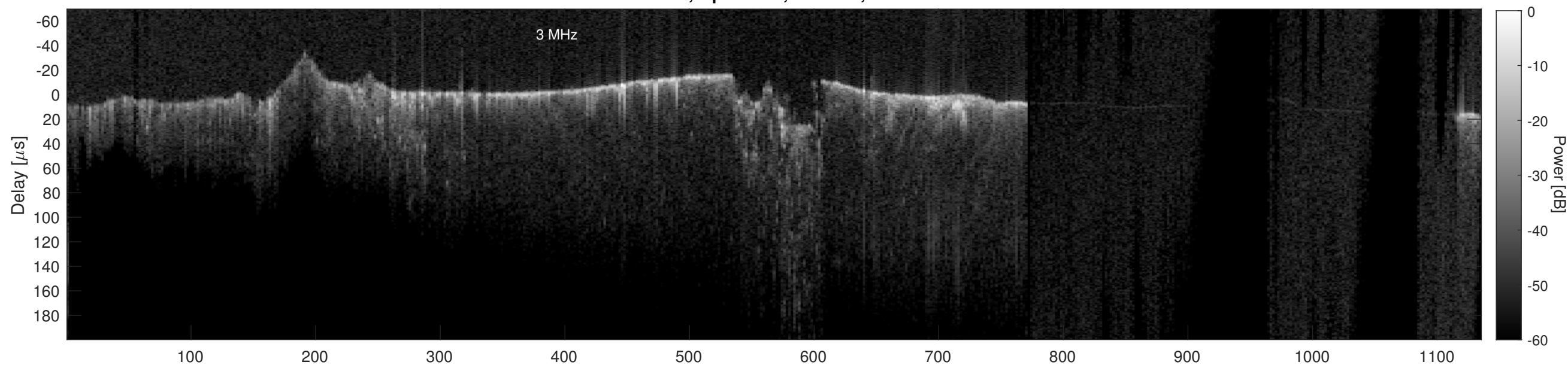
Orbit 20828, Cluttergram
