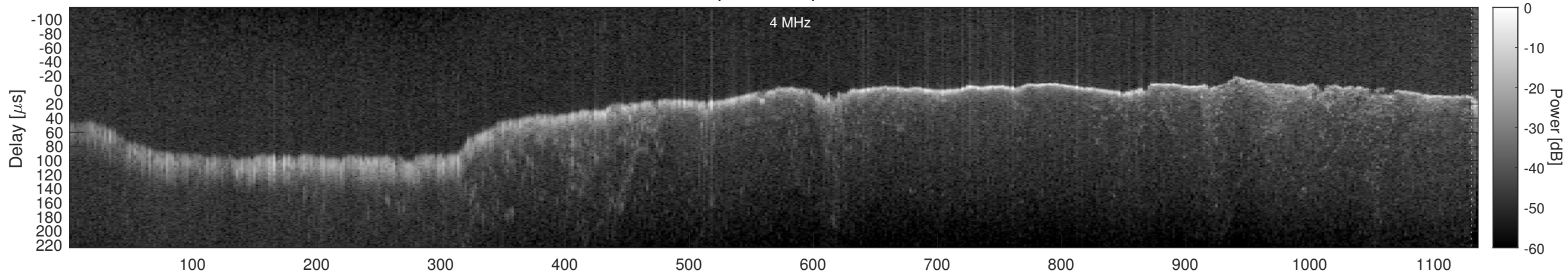
Orbit 20830, Window, Channel 1, Chapman
