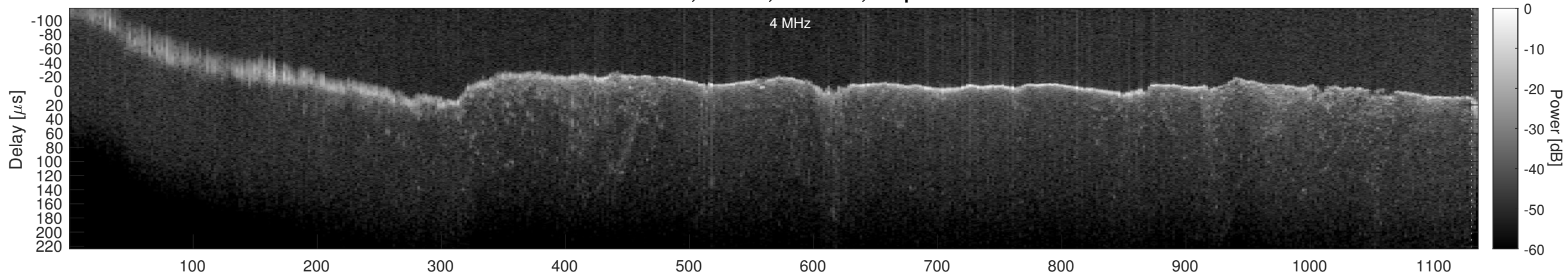
Orbit 20830, Window, Channel 1, Optimized
