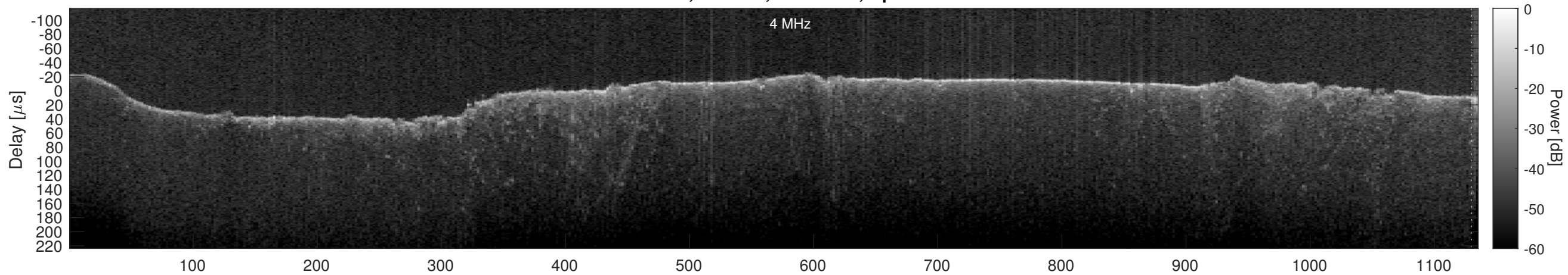
Orbit 20830, Cluttergram
