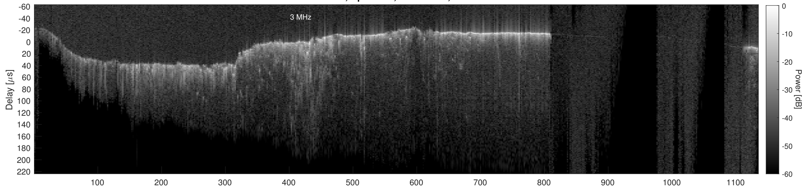
Orbit 20830, Cluttergram
