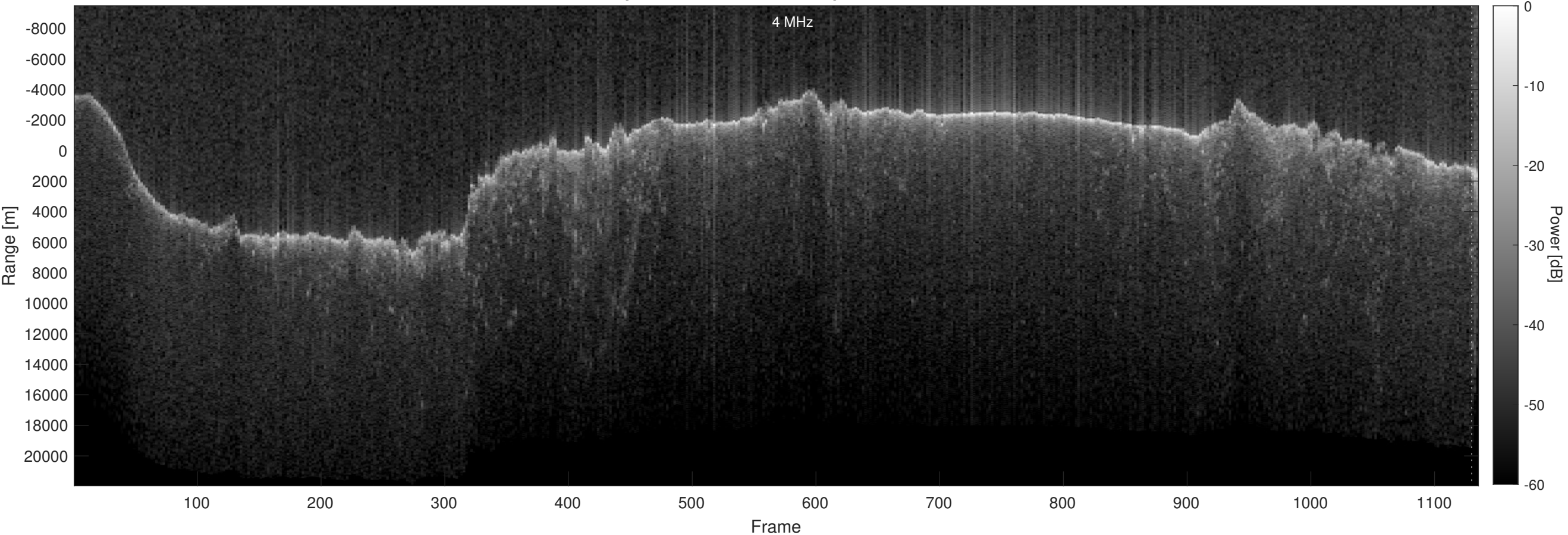
Orbit 20830, Optimized, No Window, Depth-Corrected, Channel 2
