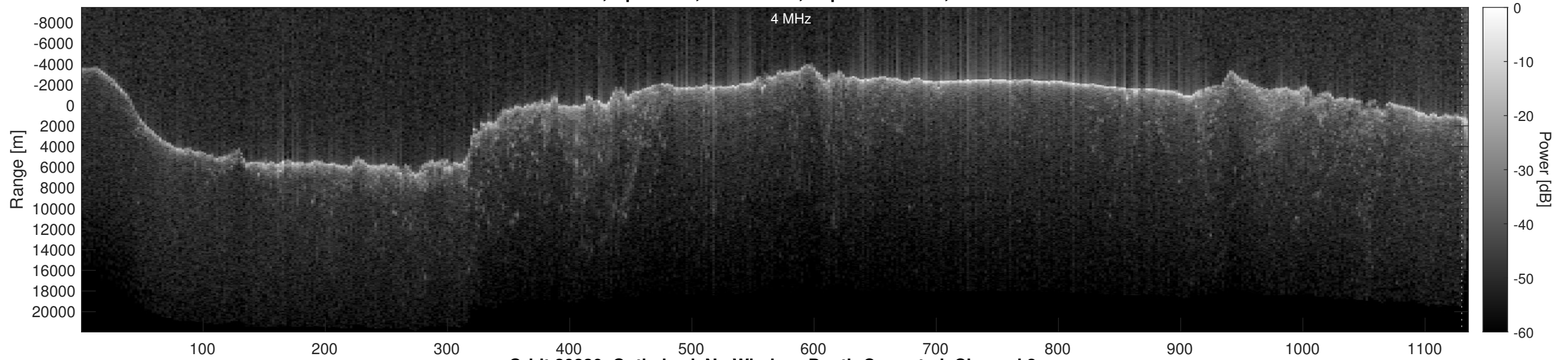
Orbit 20830, Optimized, No Window, Depth-Corrected, Channel 2
