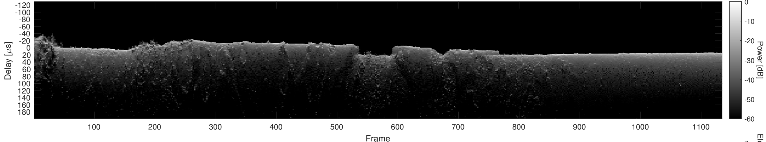
Orbit 20831, Cluttergram
