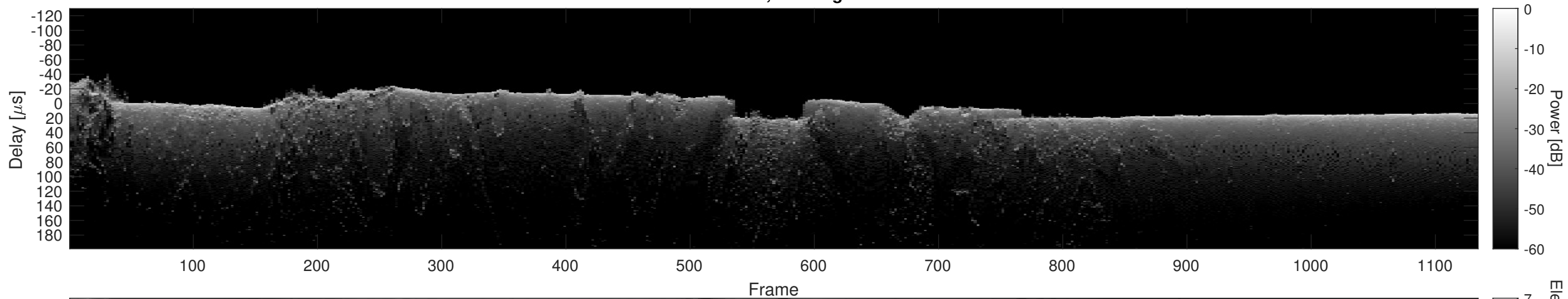
Orbit 20831, Cluttergram
