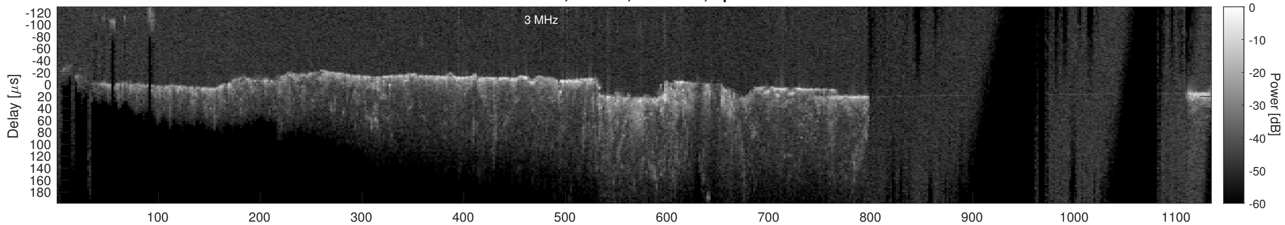
Orbit 20831, Cluttergram
