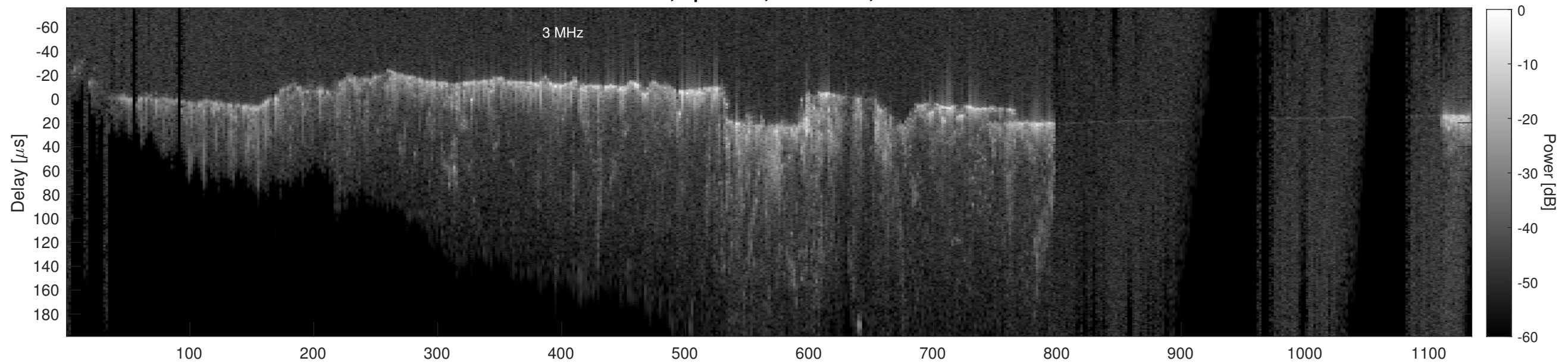
Orbit 20831, Cluttergram
