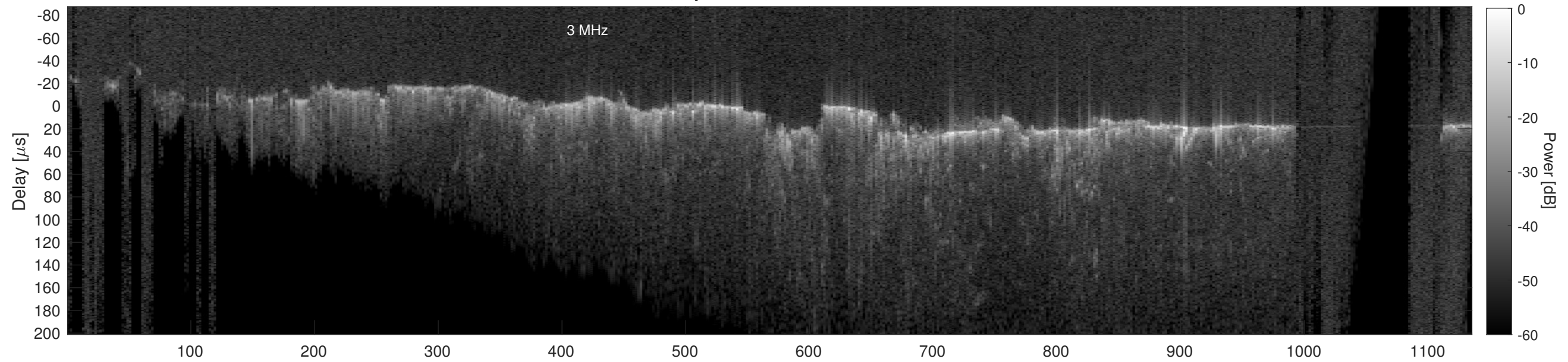
Orbit 20838, Cluttergram
