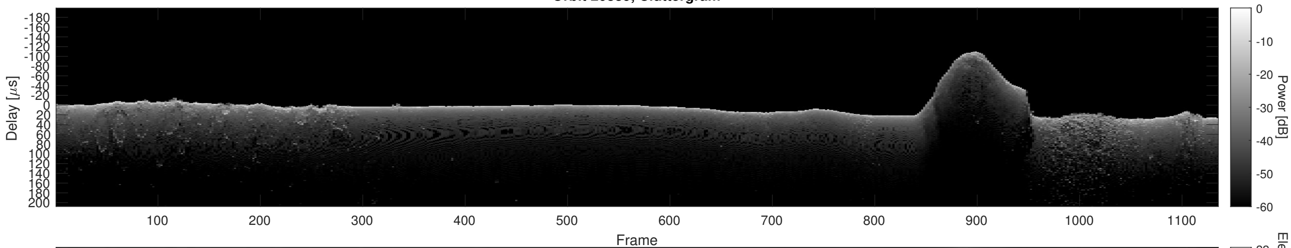
Orbit 20839, Cluttergram
