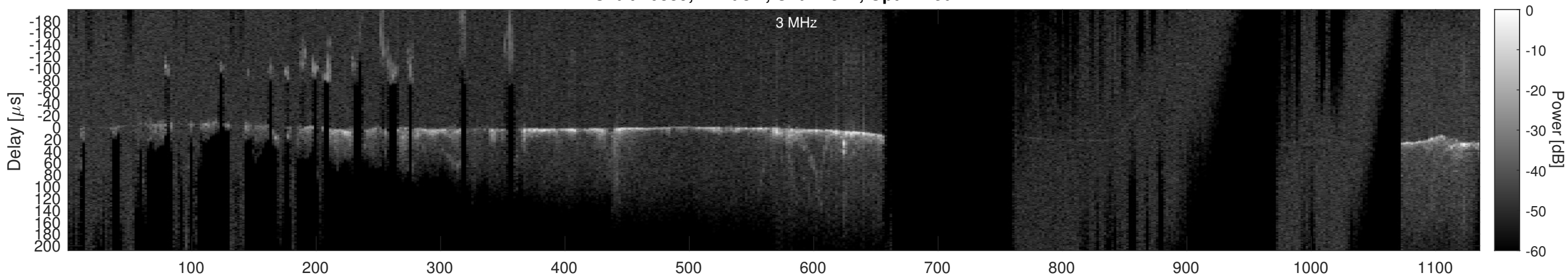
Orbit 20839, Cluttergram
