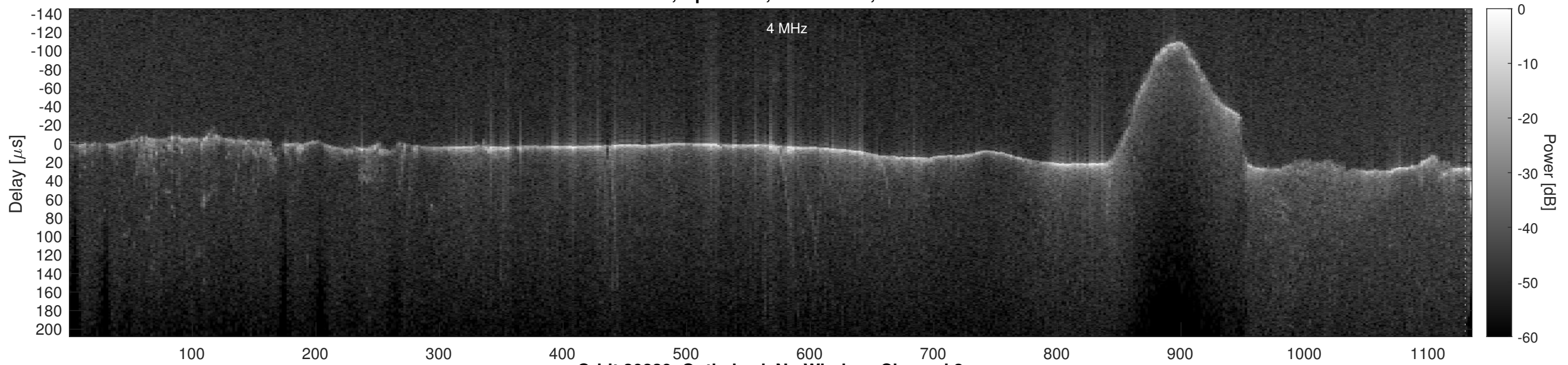
Orbit 20839, Optimized, No Window, Channel 2
