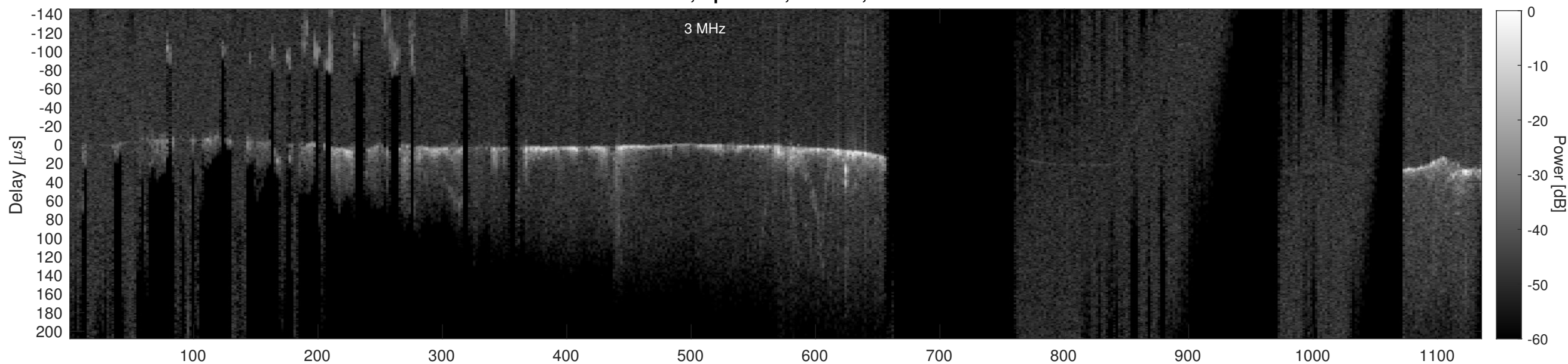
Orbit 20839, Cluttergram
