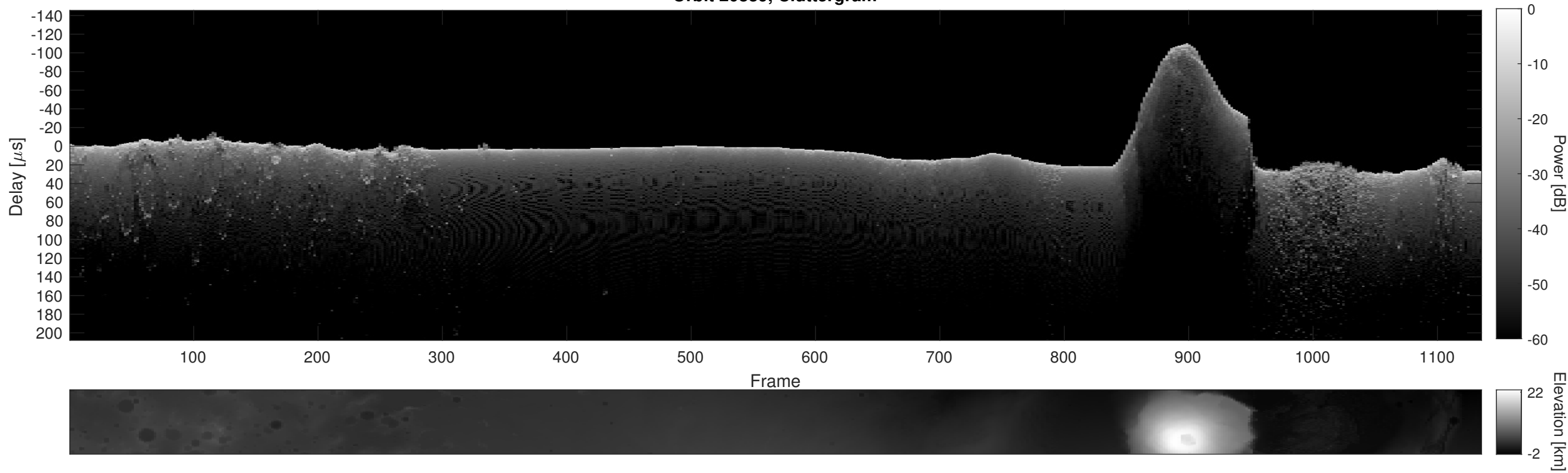
Orbit 20839, Cluttergram
