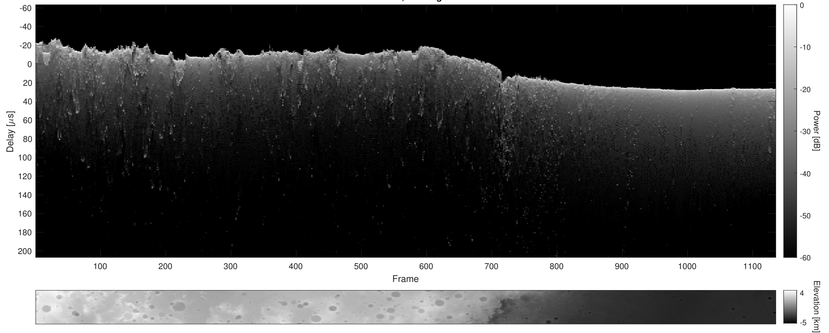
Orbit 20840, Cluttergram
