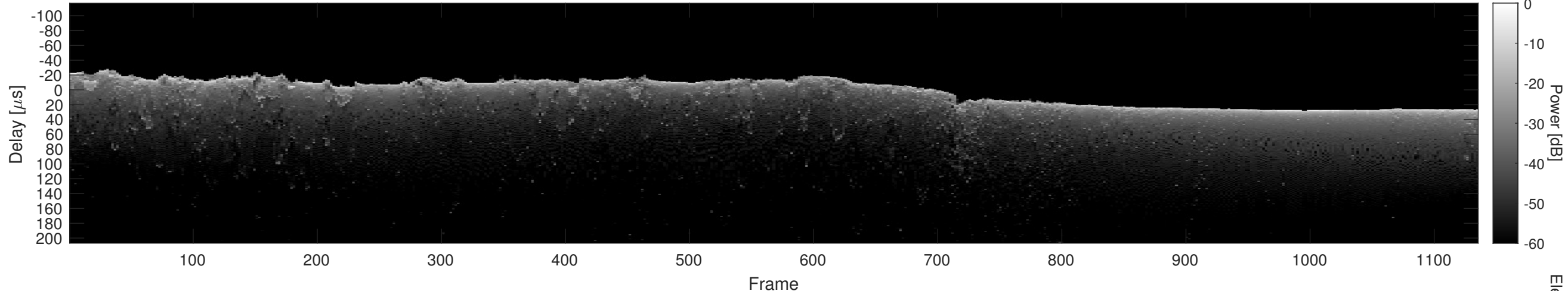
Orbit 20840, Cluttergram
