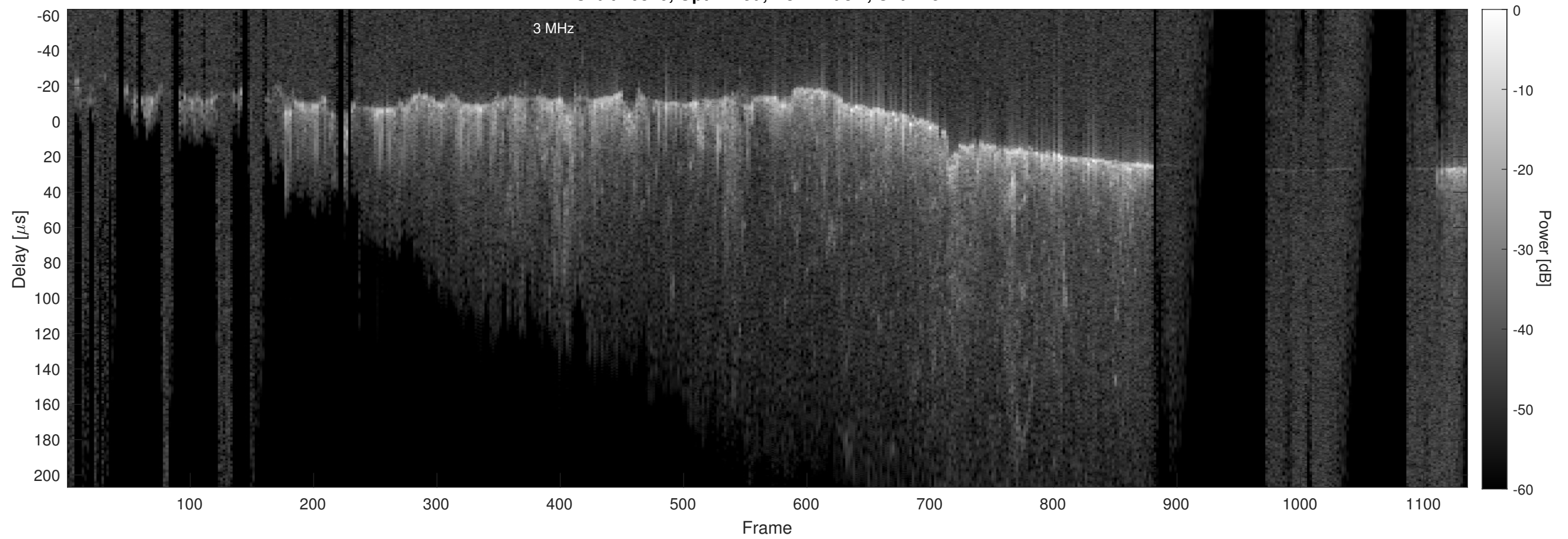
Orbit 20840, Optimized, No Window, Channel 2
