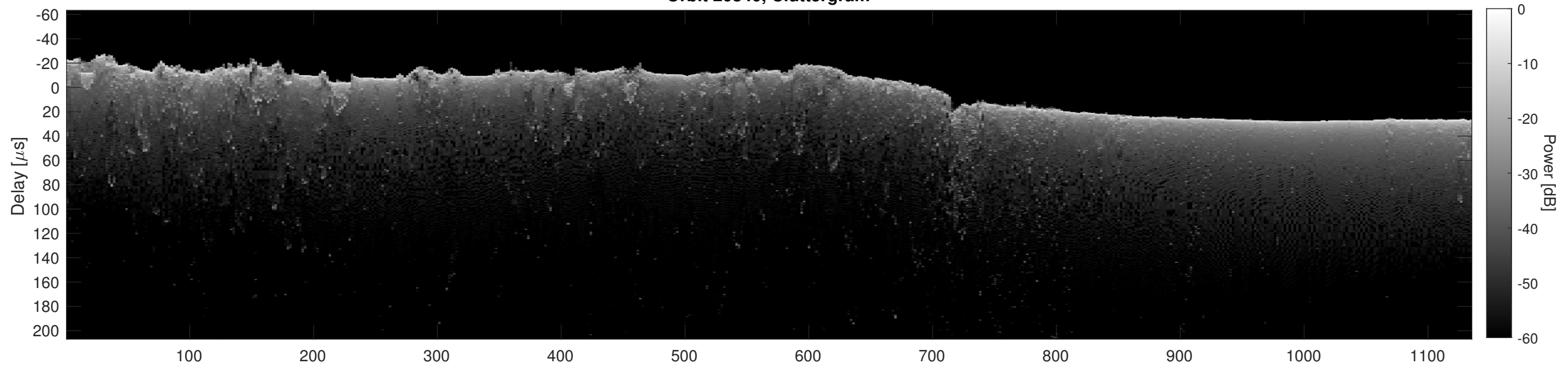
Orbit 20840, Cluttergram
