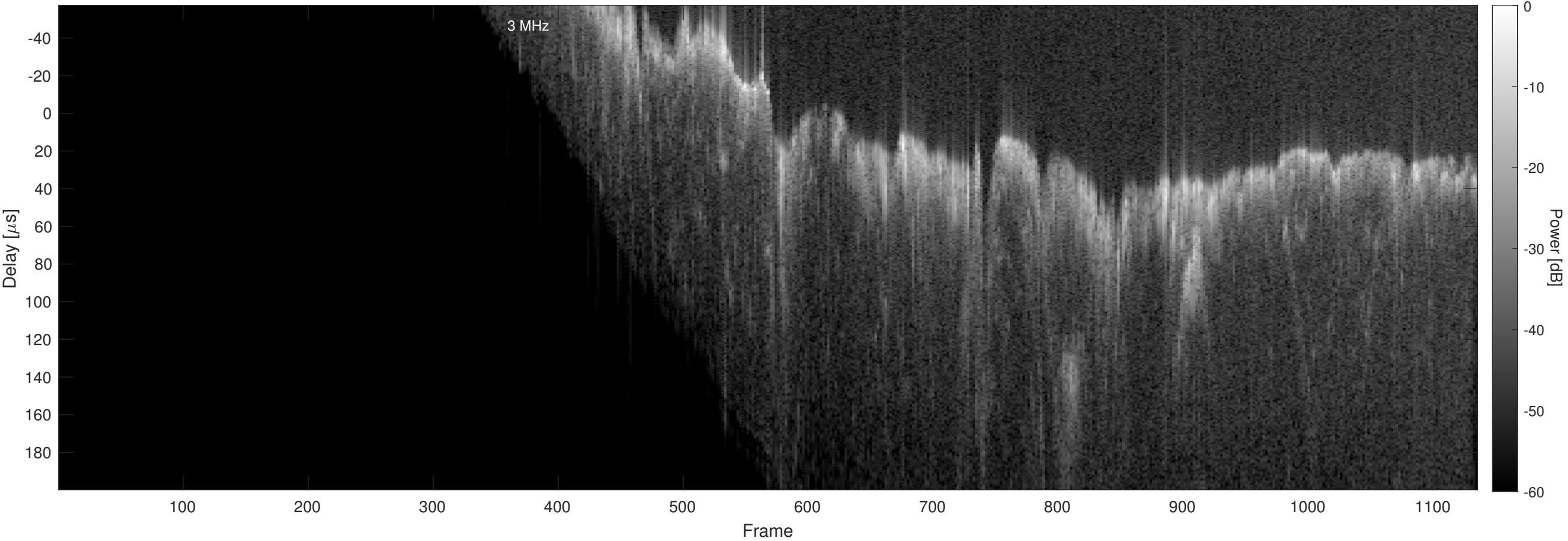
Orbit 20841, Chapman, No Window, Channel 2
